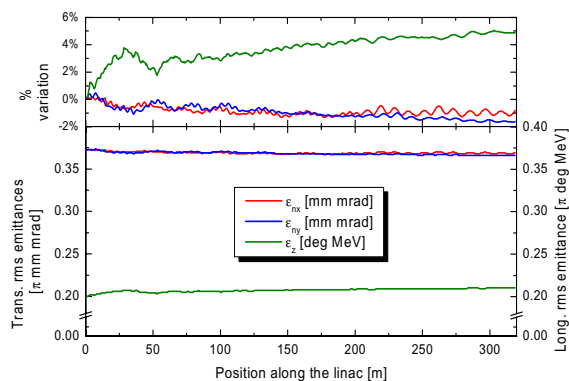
Figure 3: rms normalized emittances in the linac.
