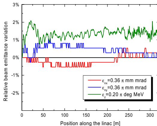
Figure 7: Relative emittance variations from PARMILA.
