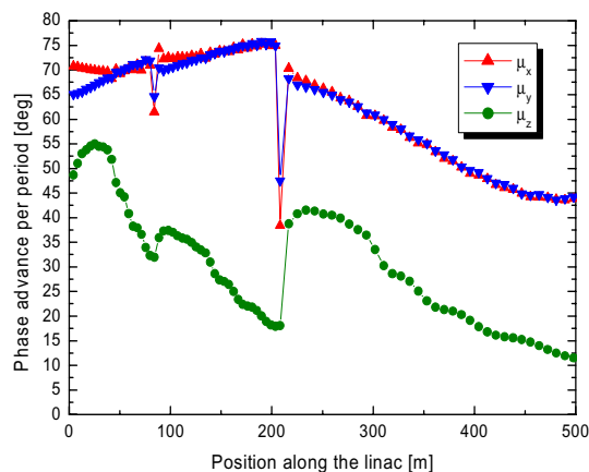
Figure 1: Phase advances for the matched beam along the 20 mA, 2 GeV SC linac.
